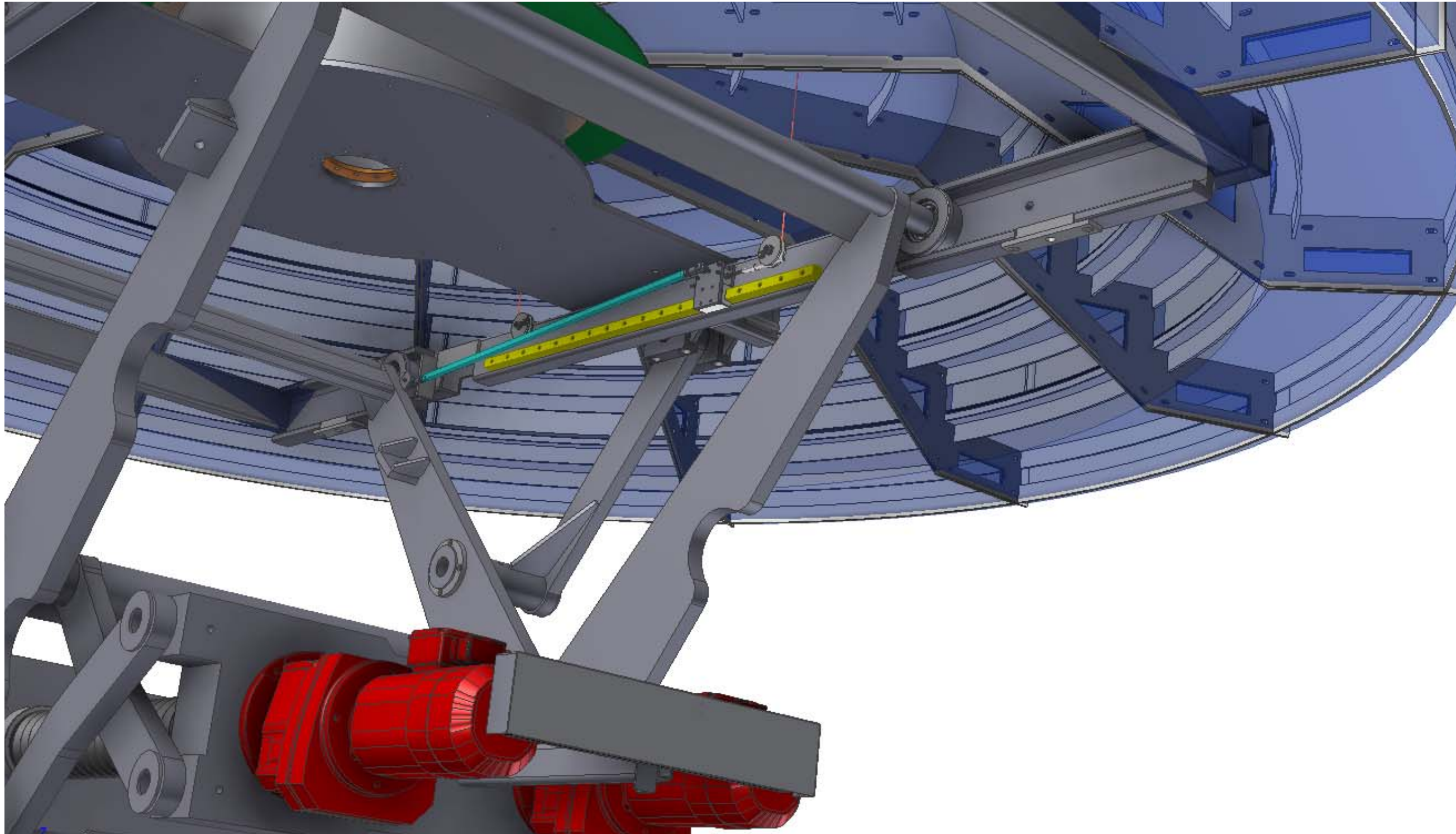
THE ELEVATOR BED COMPONENTS OF THE TURN TABLE DRIVE
